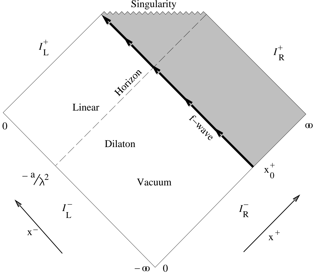
From the above we may expect that any matter perturbation of the linear dilaton vacuum will result in the formation of a black hole. To see that this is indeed the case consider the example of an f shock wave traveling in the x^- direction with magnitude a described by the stress tensor
