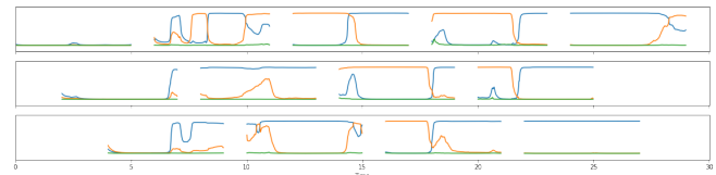
Fig. 2. Local neural speaker segmentation. For each step of the 5s window and each one of K_{\max} = 3 speakers, the segmentation model outputs the probability of the speaker being active every 16ms. We use a step of 2s between windows for readability in this figure, but the actual practical step is 500ms.
