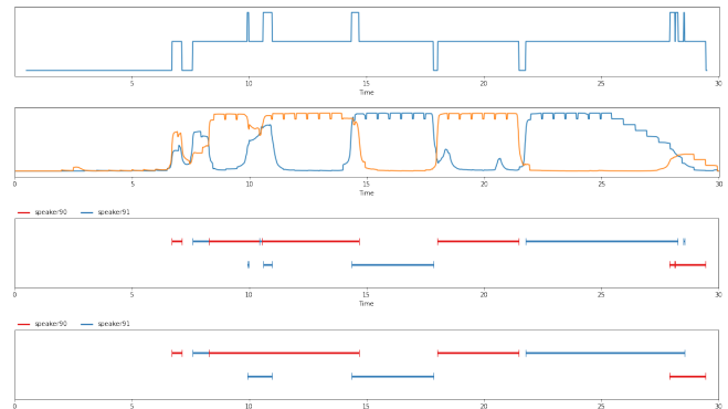
Fig. 6. Final aggregation.
