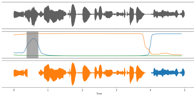
Fig. 4. Speaker embedding. Top row: 5s audio chunk. Middle row: two speakers are active according to the neural speaker segmentation model (the orange one and the blue one). Bottom row: the speaker embedding of the blue speaker is computed using only the blue audio signal, while the concatenation of orange audio signals is used to compute the speaker embedding of the orange speaker. No embedding is extracted for the green speaker as its probability never goes above \theta segmentation threshold.
