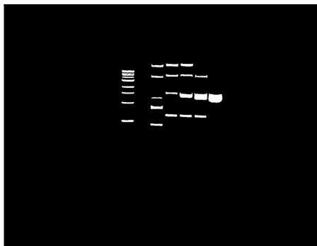
Mask Prediction
